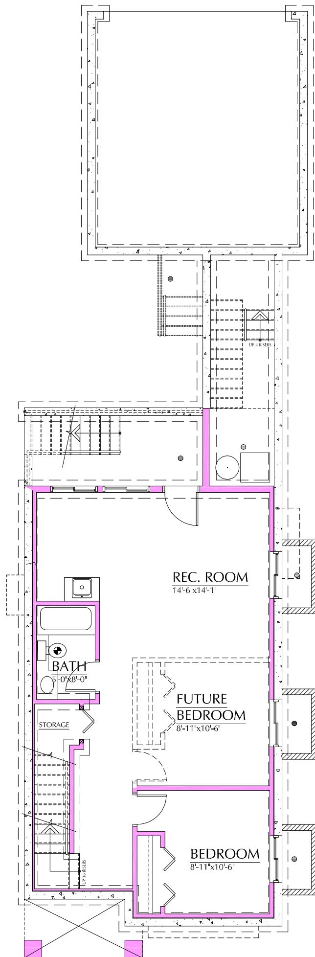
BASEMENT FLOOR BASEMENT FLOOR=849 SQ.F
